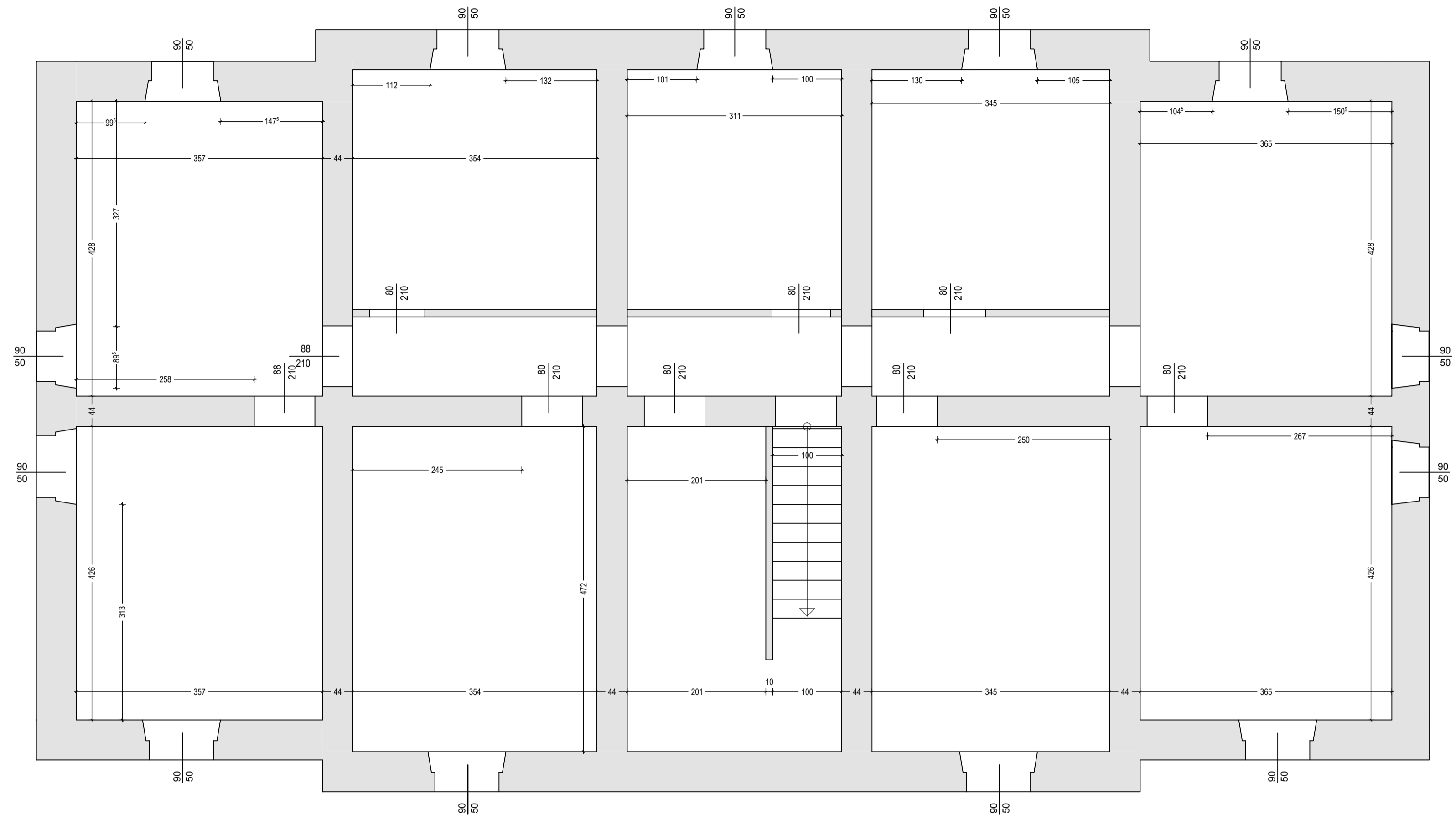
PIANO INTERRATO
